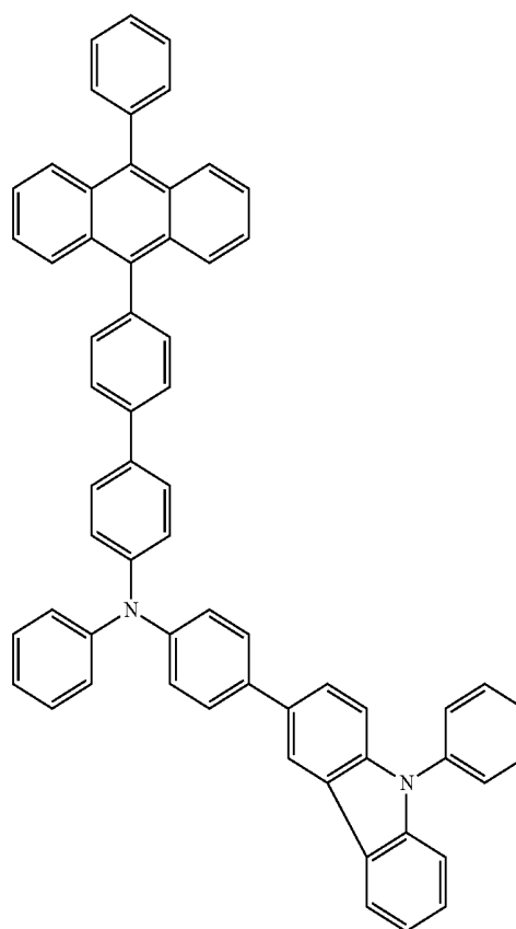
PCBAPBA
